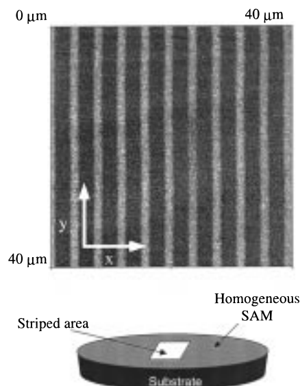
Figure 1. LFM image of the SAM substrate (40 μm × 40 μm). The substrate is topographically flat; bright stripes and dark stripes correspond to -\text{COOH} - and -\text{CH}_3 -terminated alkanethiols, respectively. The pattern periodicity is 4 \pm 0.2 μm. The schematic drawing illustrates the SAM substrates used for this study.
